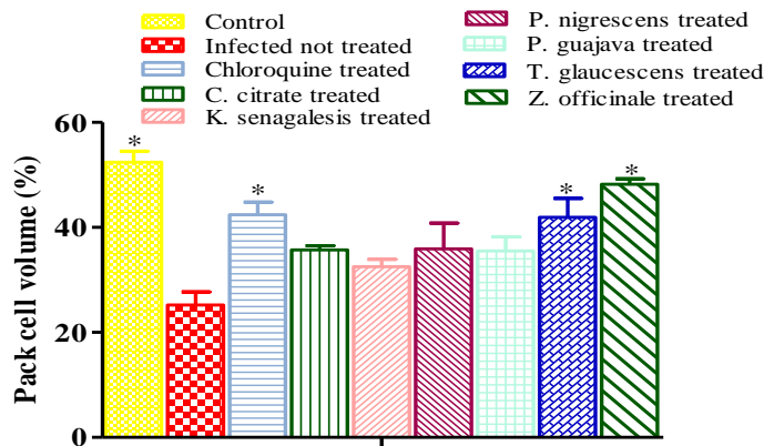
Figure 2c: Pack cell volume of P. berghei parasitized mice treated with aqueous extracts (200mg/kg bwt.) of some medicinal plant and 5mg/kg bwt chloroquine. The bars are mean \pm SEM of determinations, the * show the statistical different at P < 0.05
