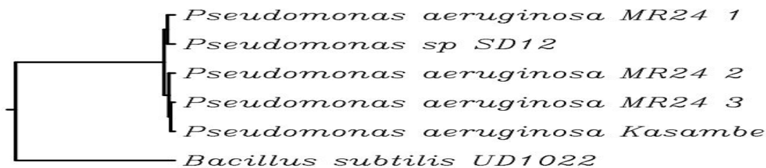
Figure 1: Phylogenetic tree of five selected Pseudomonas isolates
