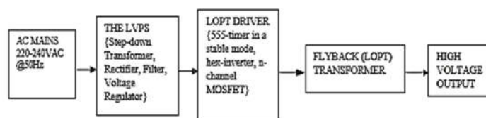
Figure 2: HVPS block diagram
