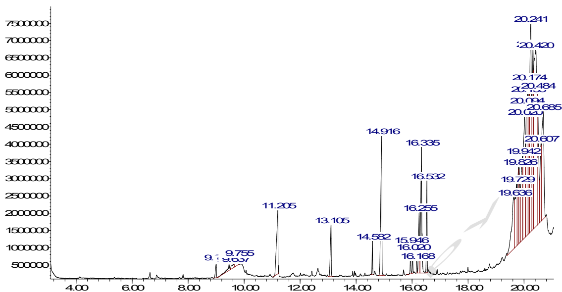
Figure 1: Total ion current chromatogram of Secamone afzelli leaves extract
